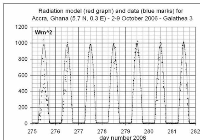
Fig. 3: The Galathea Expedition provided a unique opportunity to measure global solar irradiance over a wide range of locations, solar elevation angles and temperatures. The data shown was measured using a Sol-Data 80spc pyranometer. It was continuously checked against a second 80spc and with a Kipp-Zonen CM-11 pyranometer. Sunny days were by far the predominant weather type during the 8 month 100.000 kilometer voyage.
